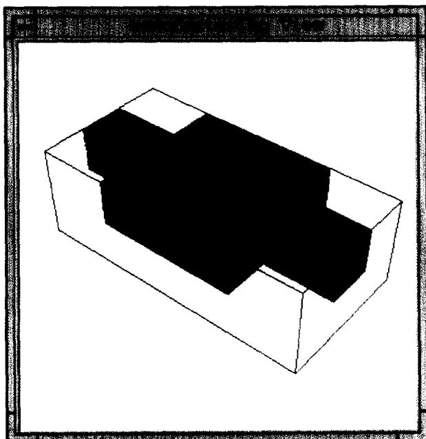
Figure 11 Feature interactions
