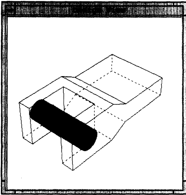
Figure 10 Non-boundary faces
